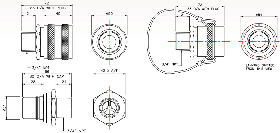
AUS27W & AUS29W shown with optional Caps/Plugs
